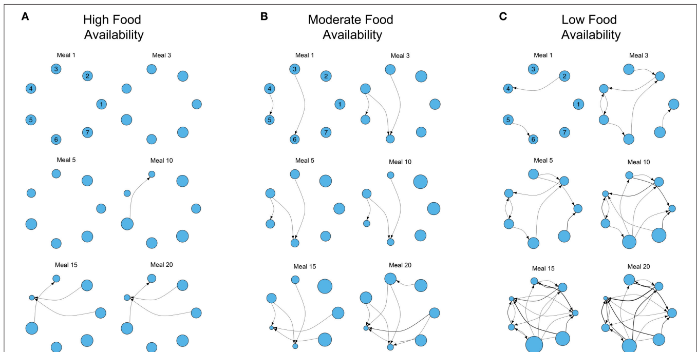
FIGURE 2 | Examples of the development of three different dominance networks in three different nutritional environments containing three foods (identical to Figure 1A) at (A) high, (B) moderate, and (C) low food availability after 1, 3, 5, 10, 15, and 20 meals, in groups of 7 individuals. Each network is directional and weighted. Each node represents 1 of 7 individuals, and the plotted position of each individual remains constant across meals in each environment (individual identities are given for meal 1). Edges represent contests, with the direction of the edge denoting the victor of the contest and the loser (recipient). Edges are weighted by the number of contests. The size of each node represents individual fitness relative to the rest of the group (larger nodes denote fitter individuals, that have nutritional state closer to the IT). The degree of food availability equates to a “competition intensity” ( c ) of 0.4, 0.6, and 0.8, as described in Senior et al. (2015a). The script is available in Supplementary File S2.
