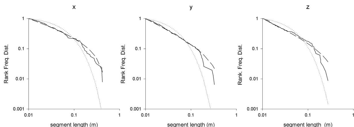
Figure 6. Rank frequency distributions of flight-step lengths tend to show near isotropic looping power-law scaling indicative of fast simulated annealing. Rank frequency distributions for bee w11 made during its first foraging bout and in the presence of large flowers (solid-lines), and shown together with the best fit power laws (dashed-lines) and best fit exponentials (dotted-lines). The Akaike weights for power-law scaling being the better scaling are all 1.00 and the maximum likelihood estimates for the power-law exponents are 1.46, 1.73 and 1.69 for the x-, y- and z-directions. The numbers of flight-steps are 126 (x), 155 (y) and 115 (z).
