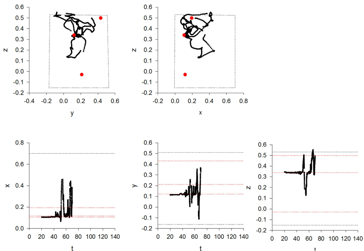
Figure 3. Partial recording of a flight pattern showing details of looping characteristics indicative of fast simulated annealing together with the time courses of the x-, y- and z-position coordinates. This looping is not evident when the entire flight pattern is plotted because it fills most of the space. The example flight pattern (bee b66 on bout 4) (●) has been projected onto the y-z and x-z planes. The flight patterns are confined by the borders of the flight arena (black dotted lines) and take place in the presence of three large flowers (●, red dashed-lines). In this example only one flower is found.
